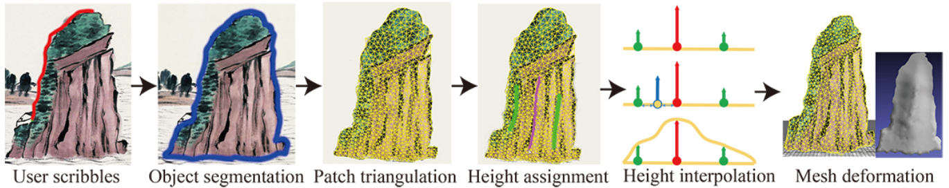
Fig. 5: This shows the construction procedure of a 2.5D scenic object. Our system lets a user select scenic objects with our implemented Intelligent Scissors [18], construct corresponding meshes using constrained Delaunay triangulation, and deform these meshes with user specified depth assignment to form the 2.5D scenic objects.
