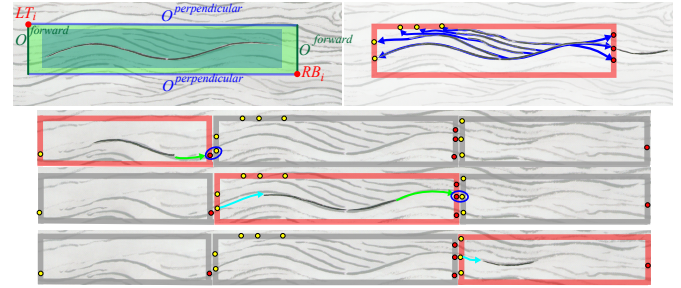
Fig. 9: This shows the process of identifying the destined region of pattern groups, registering strokes with its corresponding destined region to determine flow-in and flow-out valves (yellow and red dots), and connecting consecutive destined regions by pairing neighboring valves based on the flow field.
