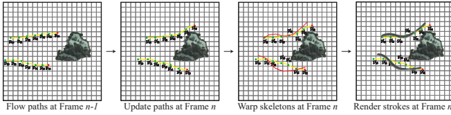
Fig. 10: This illustrates the process of advecting and animating the stroke with the flow field. The end control point of the flow path is advected with the flow field and the rest of control points take the location of its consecutive descendant control point. The skeleton path and flesh is deformed based on the newly deformed flow path coordinate described by Hsu et al. [20].
