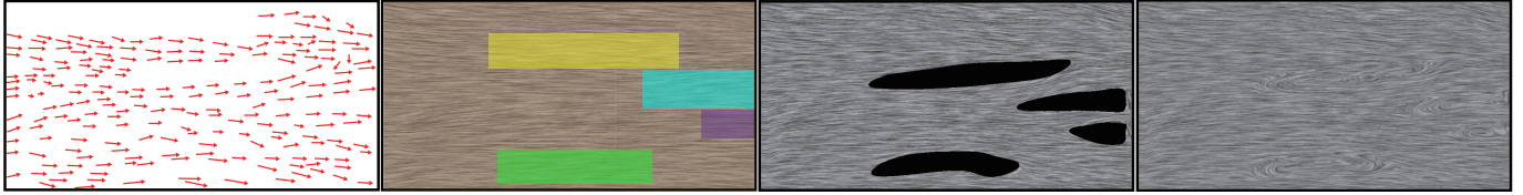
Fig. 8: These are the intermediate flow-field generation results from “Red Cliff” with 1) the initial velocities using extracted strokes, 2) the initial flow field interpolated from the initial velocities, 3) the flow field generated by solving the Navier–Stokes equations, and 4) the complete field after adding swirling fields computed by harmonic functions.
